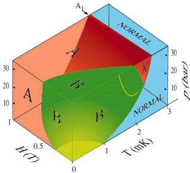
Superfluid He-3 (cf Nobel Prize 2003)
